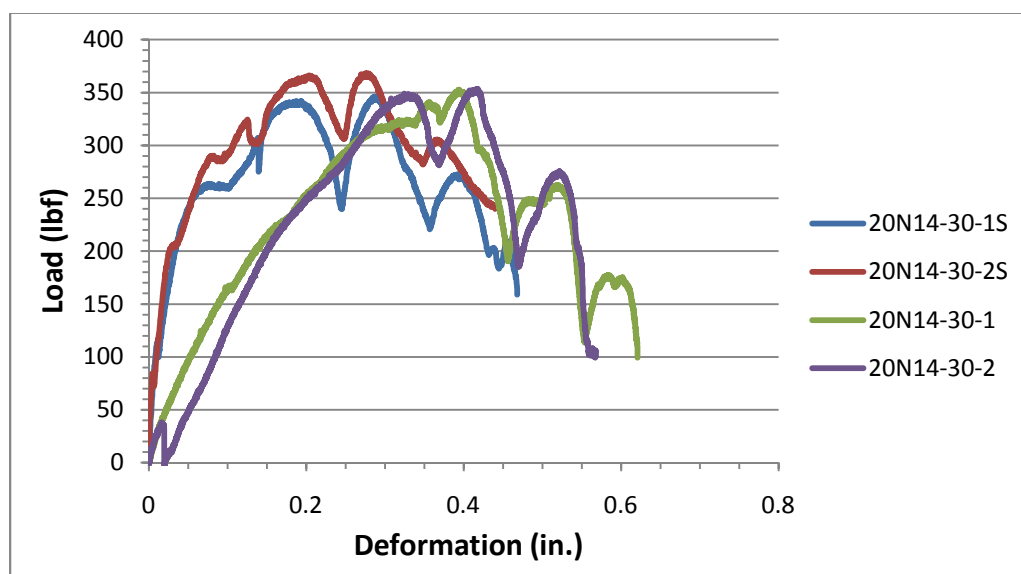
Figure 3.12 Load versus Deflection of 30° Test Specimens
